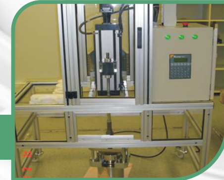
Dayanıklılık test makinesi Durability test machine
